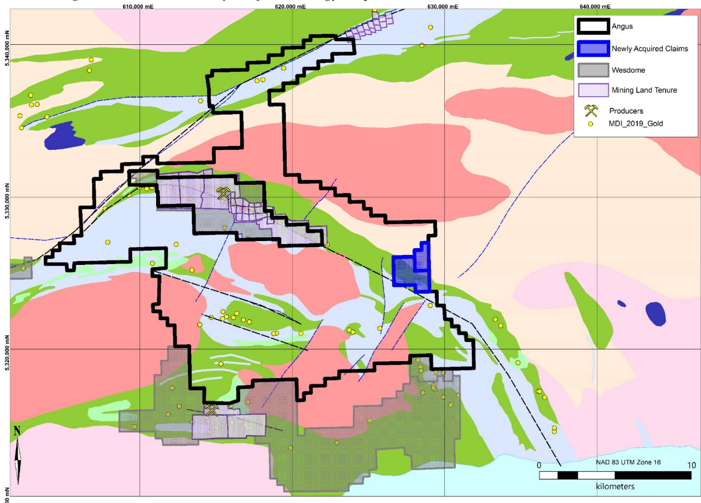
Figure 1 – The Golden Sky Project Geology Map
