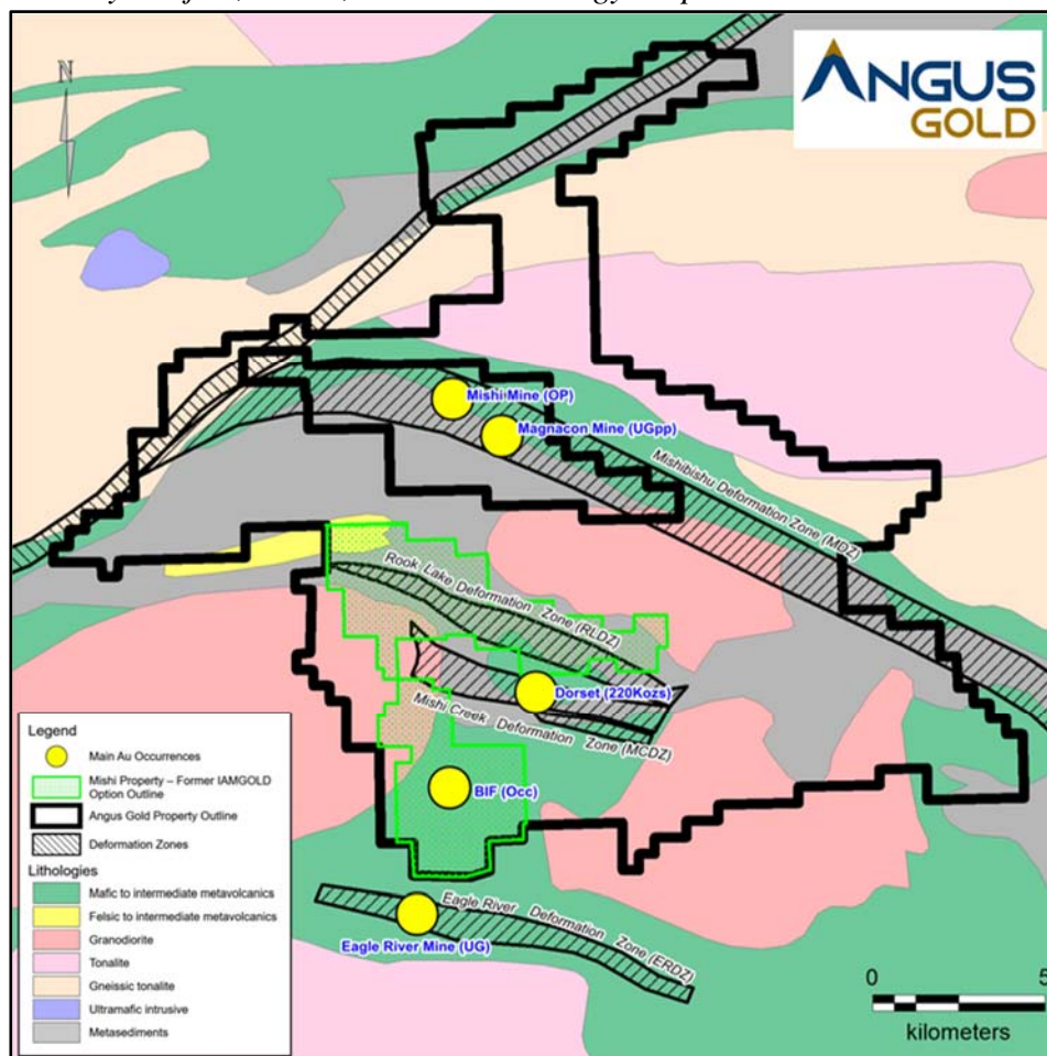
Figure 1: Golden Sky Project, Wawa, Ontario – Geology Map
